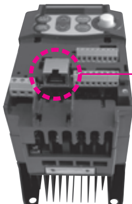
RS-485 communications connector
