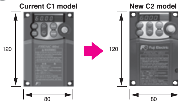
Note: Three-phase 200V 0.1–0.75kW dimensions shown (mm)
